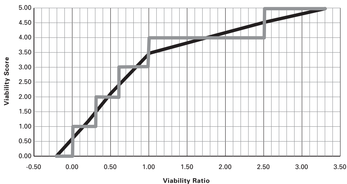
Figure 1. Viability Scores
